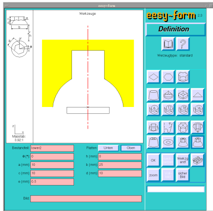
Fig 10 Input mask showing the various tool shape generation module
